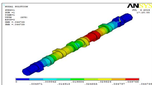
Fig -5: Displacement of cam
