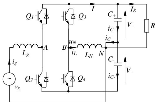
Figure 1. The single-phase rectifier under investigation.
