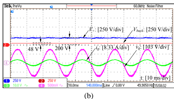
Figure 15. System performance with a buck DC/DC converter and a resistor as the load of the rectifier.
