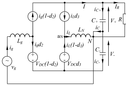
Figure 2. The average circuit model of the rectifier shown in Figure 1.
