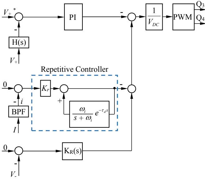
Figure 3. Controller for the neutral leg.
