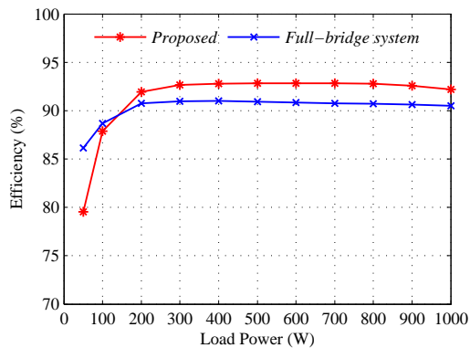
Figure 17. Efficiency comparison.
