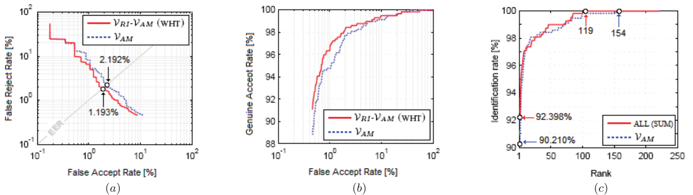
Fig. 3. Results of multimodal open/closed set identification system. (a) The ROC curves, FRR against FAR, with respect to the unimodal and multimodal systems, (b) The ROC curves, GAR against FAR, with respect to the best case and (c) The CMC curves with respect to the unimodal and multimodal systems.
