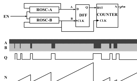
Fig. 1: Architecture of single phase BFD-TRNG [3].
