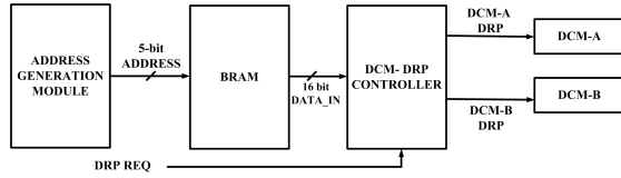
Fig. 3: Architecture of tuning circuitry.
