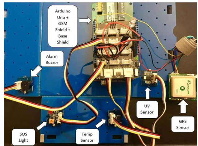
Fig 2. Proposed wearable IoT Device.
