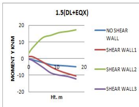
4.3.c: Graph of Bending Moment Y
