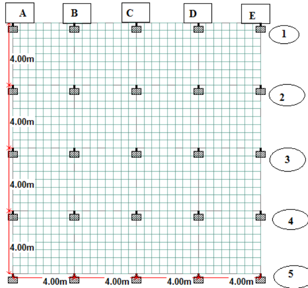
Fig. 1 Model of Building Without Shear Wall.
