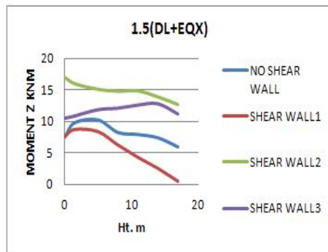
4.4.d: Graph of Bending Moment Z
