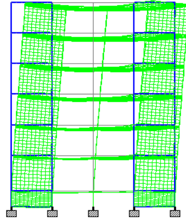
Model II: Structure with L type shear wall
