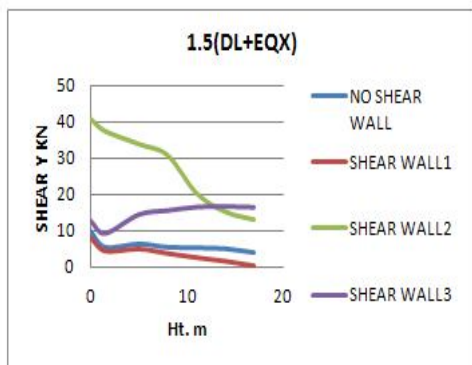
4.1.a: Graph of Shear Force Y
