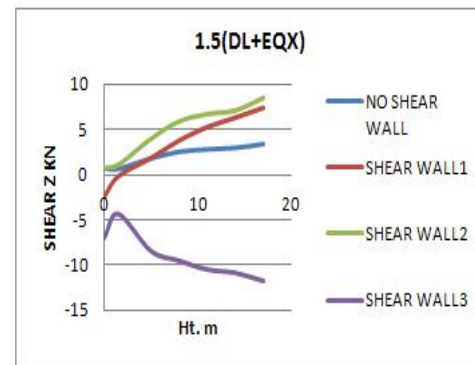
4.2.b: Graph of Shear Force Z
