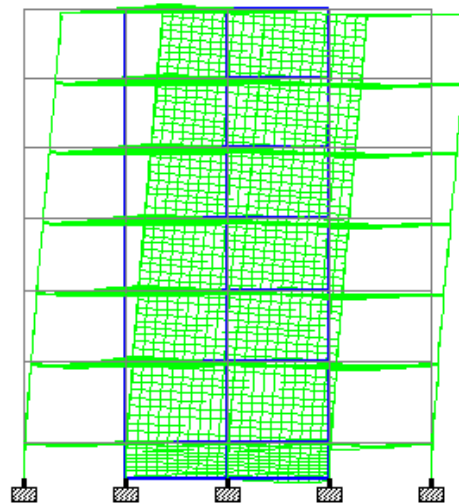
Model IV: Structure with cross type shear wall
