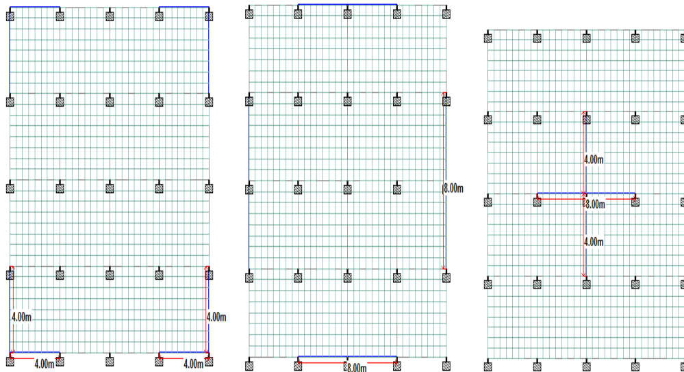
Figs: Different model of building with different type of shear wall.
