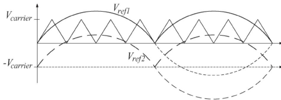
Fig.1 Carrier and reference signals
