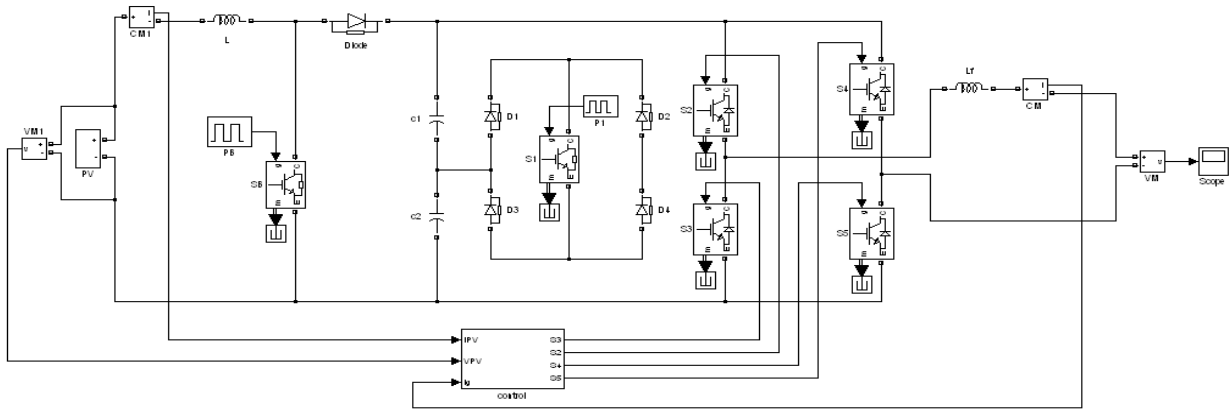
Fig.4 Simulink diagram for five level inverter
