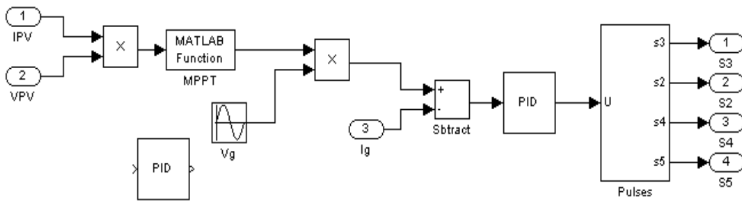
Fig.5 MPPT technology
