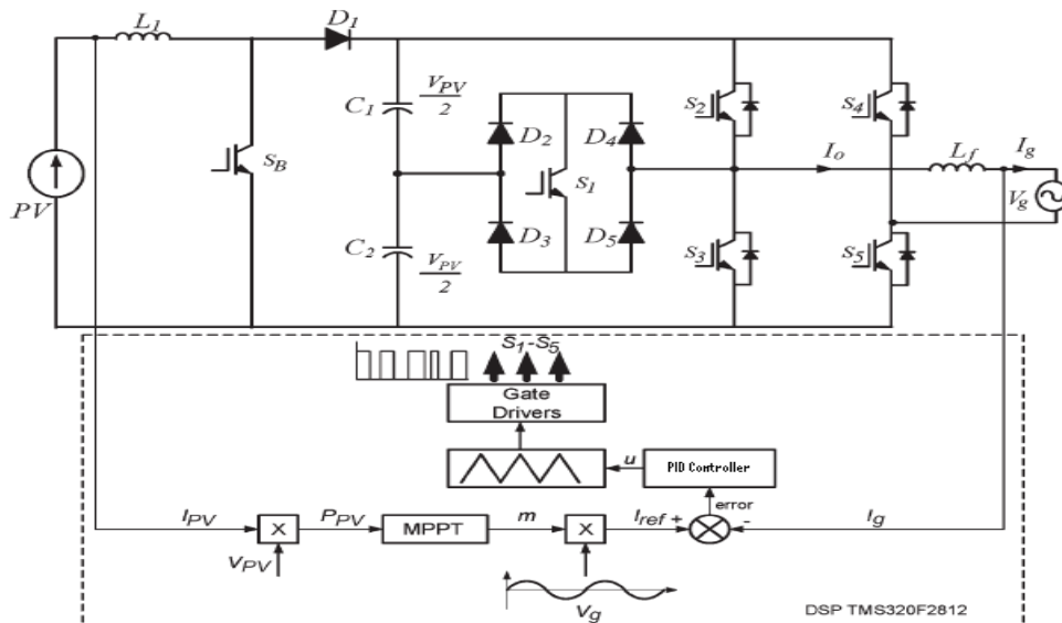
Fig.3 Five level inverter with control algorithm implemented in DSP TMS320F2812
