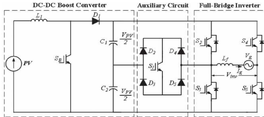
Fig.2 Single phase five level inverter topology
